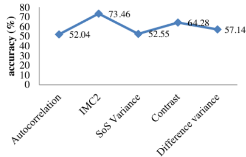
Figure 6. Graph of identification of accuracy percentage of each input feature in neural network
