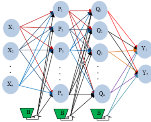
Figure 3. NN architecture
