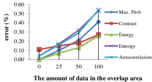
Figure 5. Graph of error percentage based on the amount of data in overlapped probability range area
