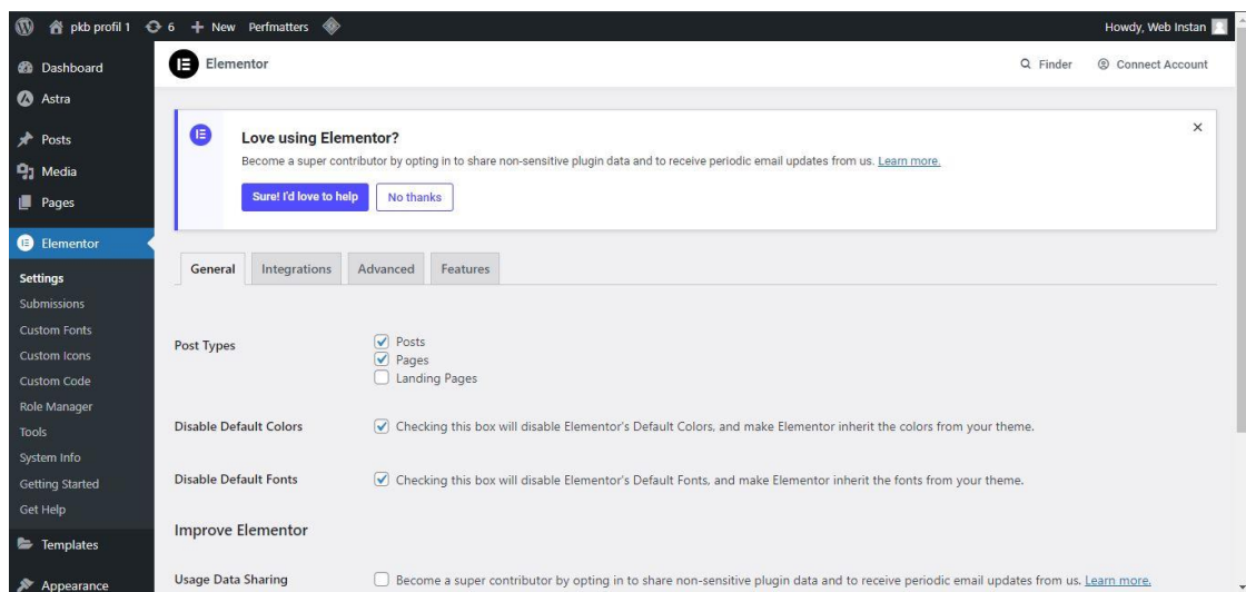
Gambar 3. 1 Tampilan WordPress
