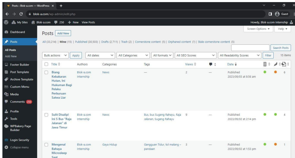
Gambar 3.5 Halaman All-Post
