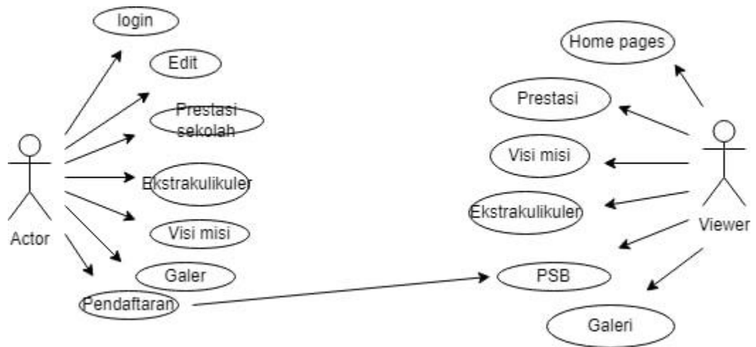
Gambar 3 . 1 Gambar Use Case Diagram
